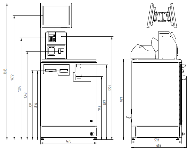
Semi Note Recycling, Full Coin Recycling, EFT Enabled,
